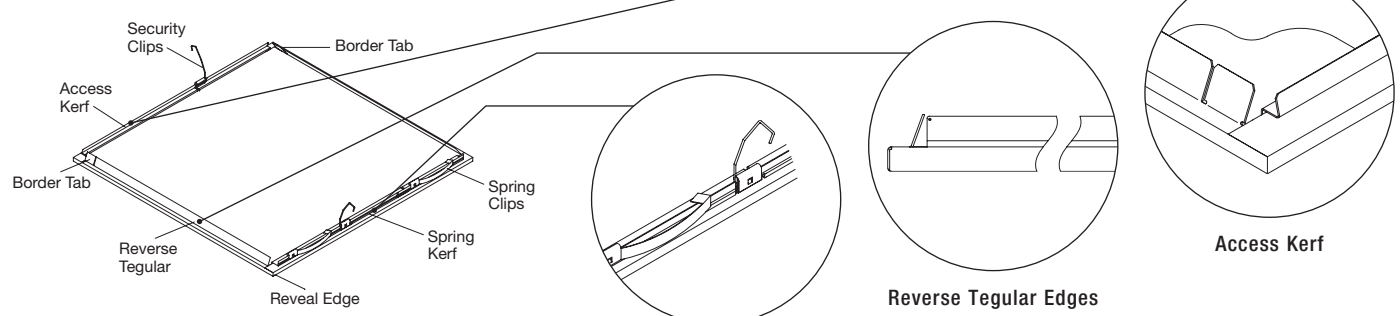
MetalWorks Vector Panel Detail
