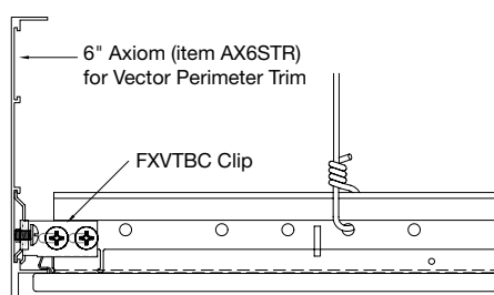
Axiom Classic Trim Application
