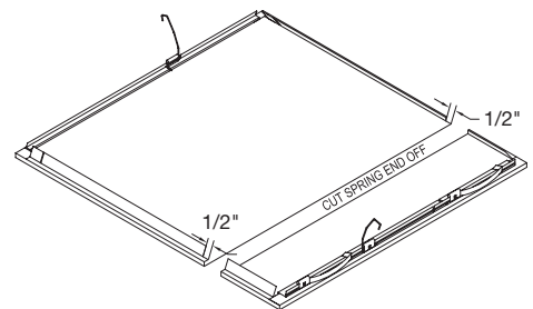
Cutting MetalWorks Panel for Edge Cap
